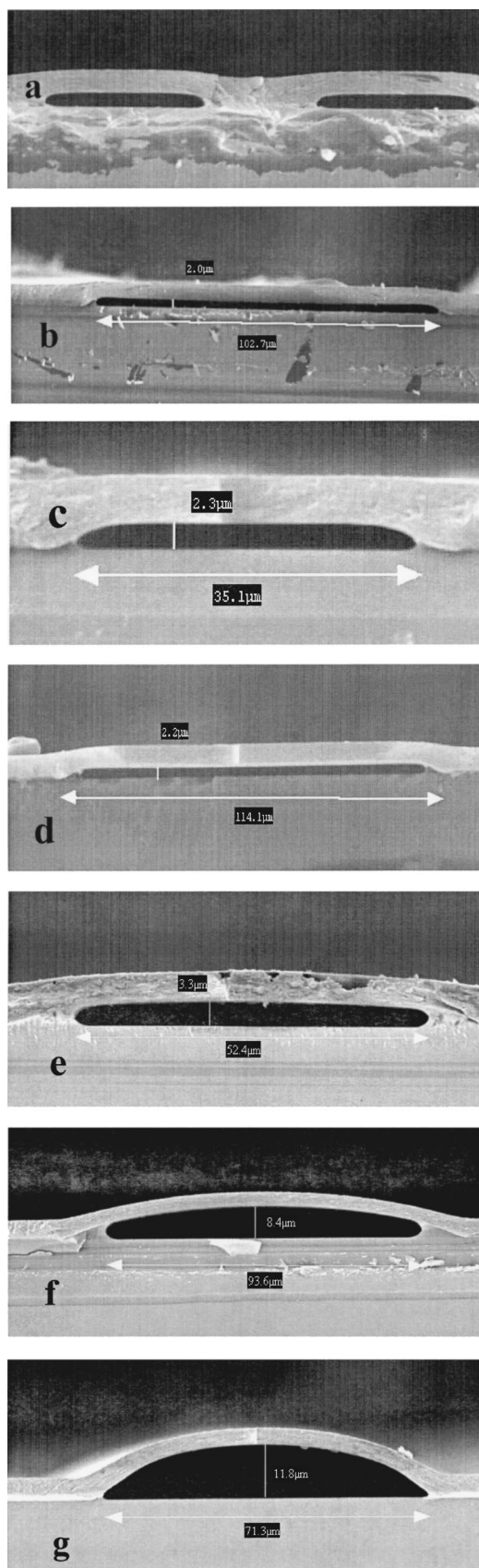
Figure 8. SEM images of the channels encapsulated with polyimide and decomposed with at rates of (a, b) 1%/min, (c, d) 2%/min, (e, f) 3%/min, and (g) at a constant 425°C.
